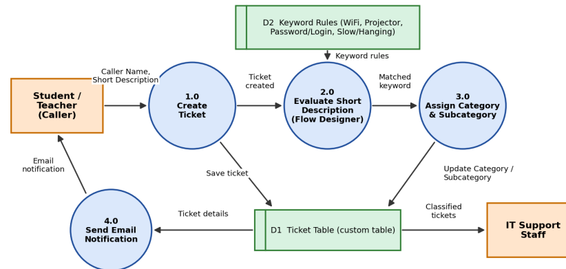
Data Flow Diagram (Level 1) - Auto Ticket Classification using Flow Designer
